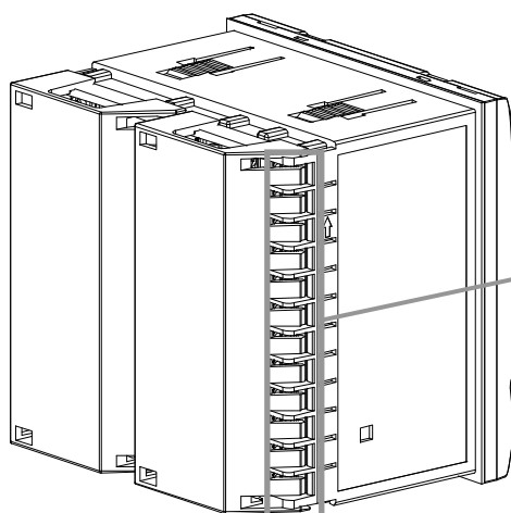
With the terminal cover fixed to FB900
